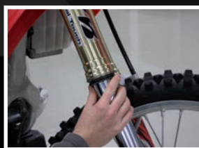
8. Slide up the dust seal
