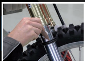
5. Apply grease on dust seal
