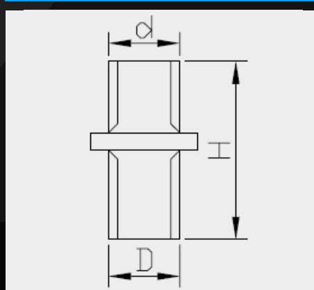
Air Valve Comp With O-ring dimensions
