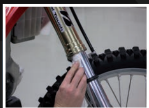
3. Clean space between the dust and oil seal
